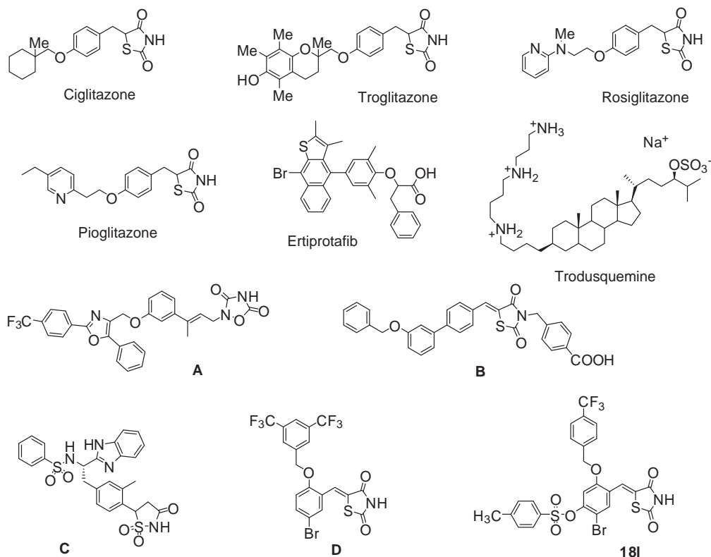
Figure 1. Thiazolidinedione derivatives and related compounds reported as PPAR- \gamma activators or PTP1B inhibitors.
