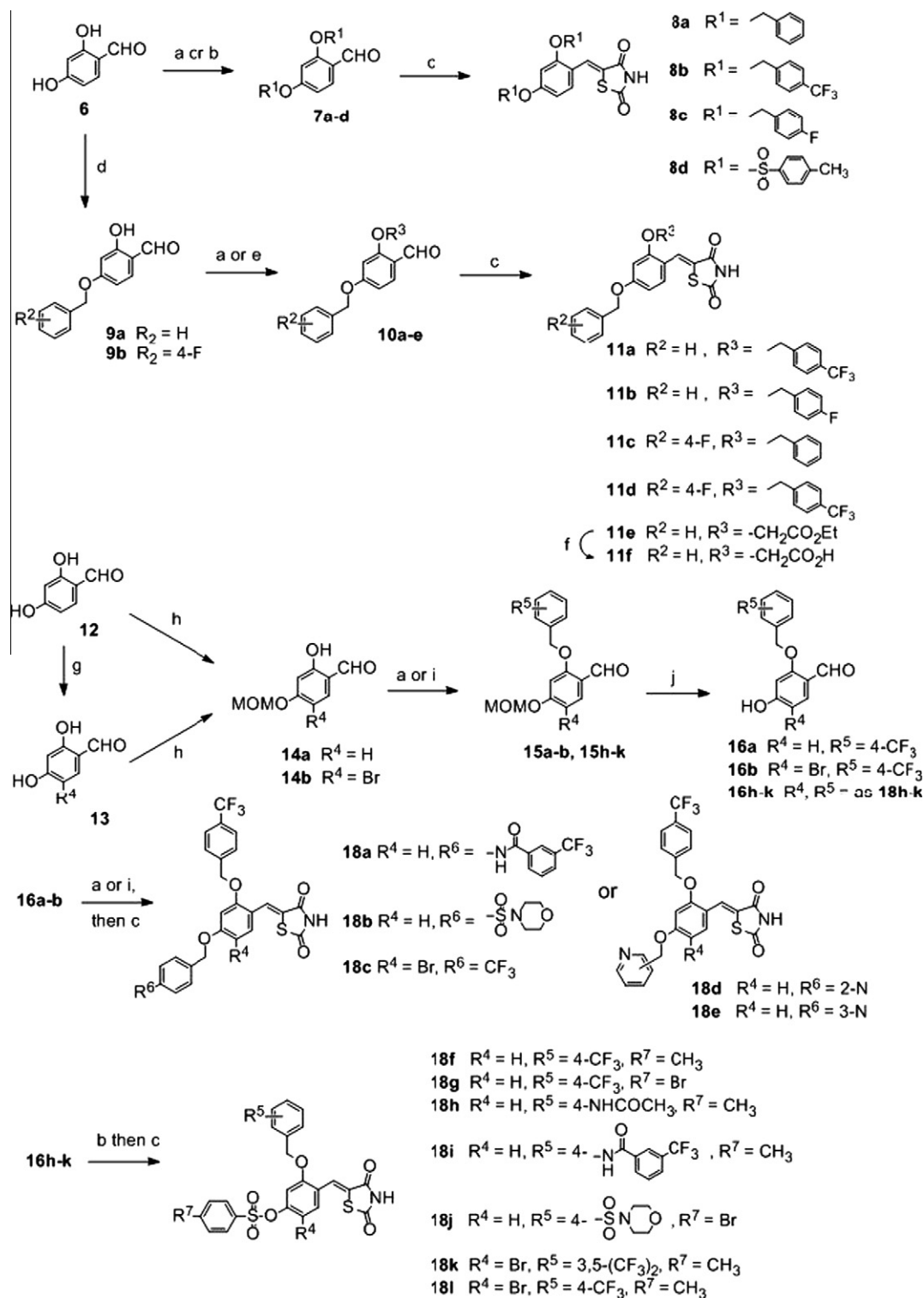
Scheme 1. Reagents and conditions: (a) RPhCH 2 Cl or RPhCH 2 Br, K 2 CO 3 , DMF or acetone, reflux, 1–3 h; (b) RPhSO 2 Cl, DIPEA, DMF, 0 °C to rt, 3 h; (c) 2,4-TZD, EtOH, piperidine, reflux, overnight; (d) R 2 PhCH 2 Cl, KI, NaHCO 3 , CH 3 CN, rt to 90 °C, 24 h; (e) BrCH 2 COOEt, K 2 CO 3 , DMF, 90 °C, 3 h; (f) NaOH, MeOH, H 2 O, 70 °C, 1 h; (g) Br 2 , CH 2 Cl 2 , 0 °C to rt, 3 h; (h) MOMCl, K 2 CO 3 , acetone, 0 °C to rt, 6 h; (i) RPhCH 2 Br, K 2 CO 3 , DMF, rt, 1–3 h; (j) THF/HCl, 50 °C, 2 h.
